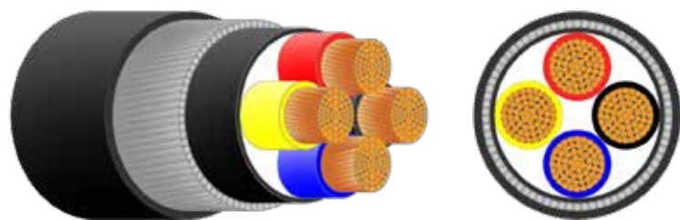
XLPE INSULATED ARMOURED PVC SHEATHED CABLE - TWO CORES CU/XLPE/PVC/SWA/PVC CABLE [IEC 60502-1, MS 2107] 0.6/1 (1.2) kV
